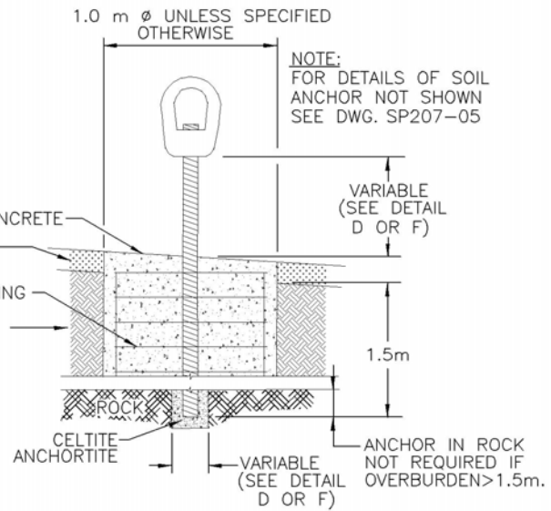
SOIL ANCHOR DETAIL ALTERNATE ANCHOR DETAIL IN OVERBURDEN. FOR OVERBURDEN THICKNESS GREATER THAN 0.6m (SEE SUBSECTION 207.01.08)
