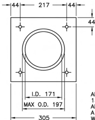
ADAPTOR PLATE
