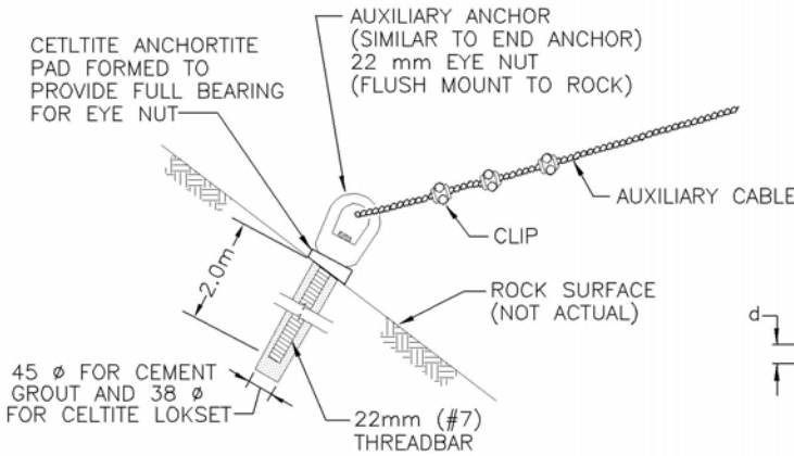
DETAIL F AUXILIARY ANCHOR CONNECTIONS
