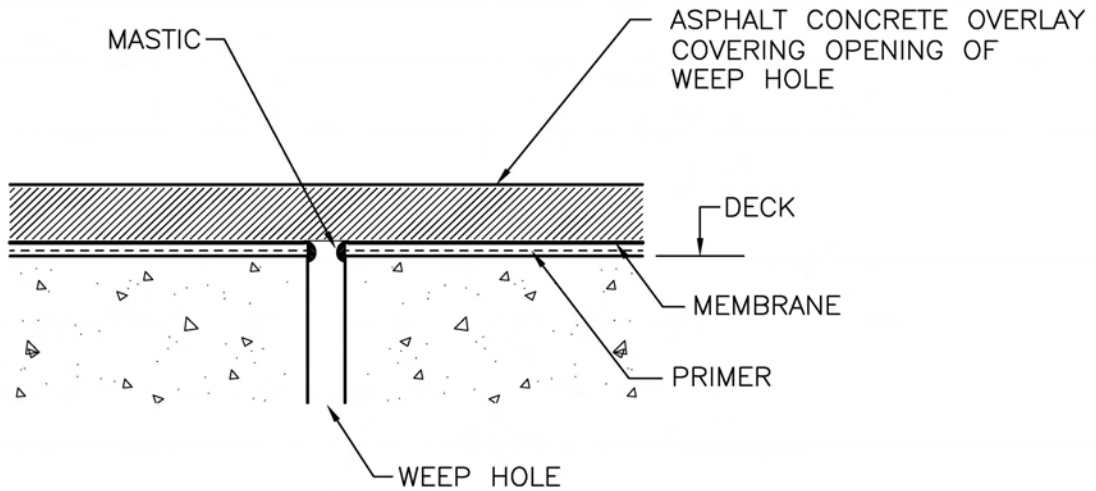
WEEP HOLE
