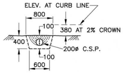
SECTION Z-Z FOR PIPE OUTFALL
