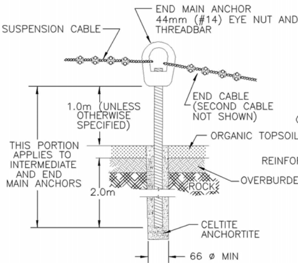
DETAIL D END MAIN ANCHOR CONNECTIONS (MESH OMITTED FOR CLARITY)
