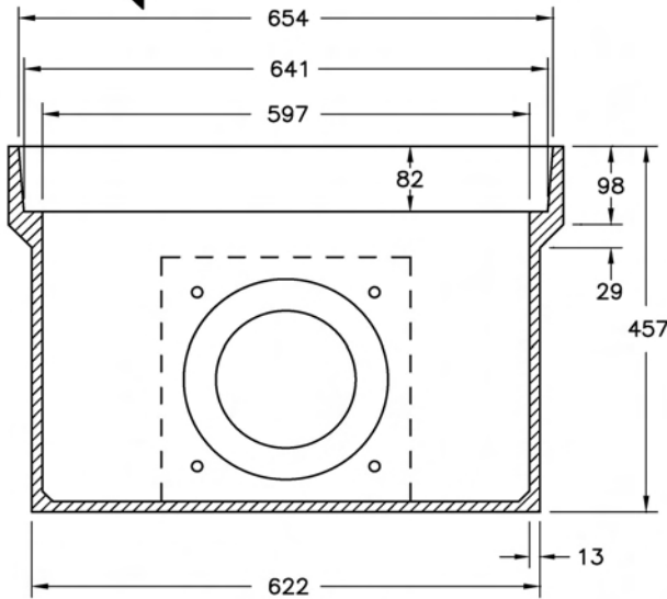
SECTION A
