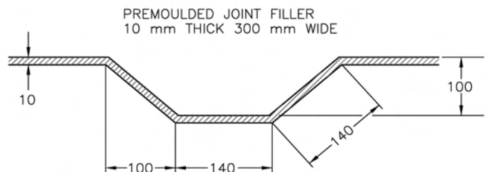
SECTION A-A EXPANSION JOINT
