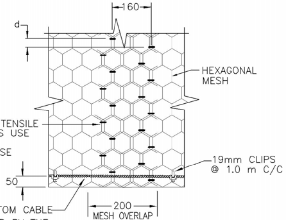
DETAIL E MESH SEAM CONNECTIONS AND BOTTOM CABLE
