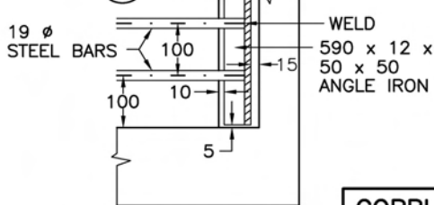
DETAIL D
