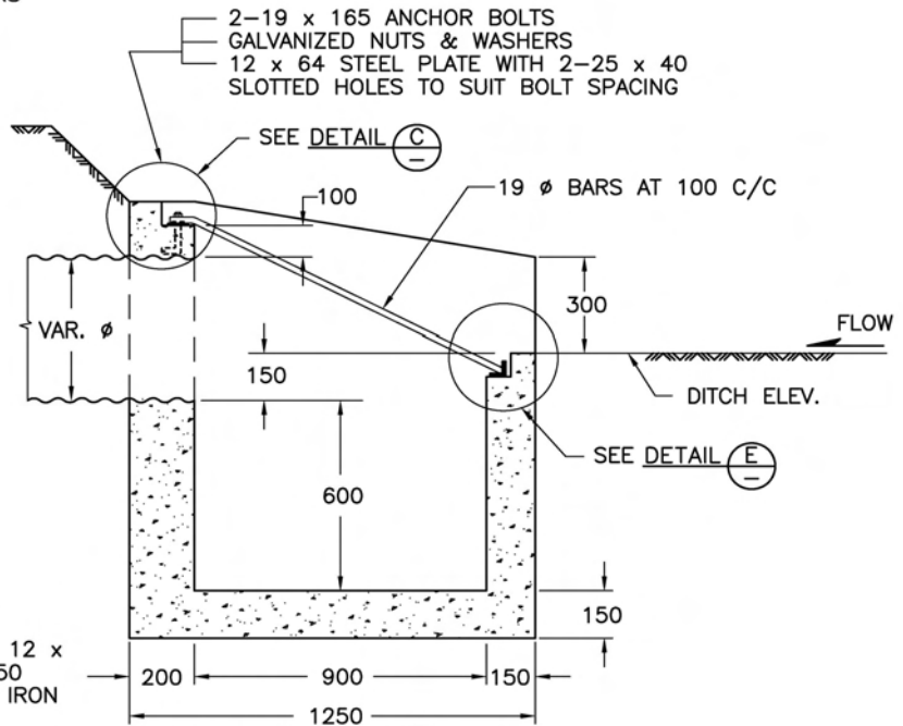
SECTION A
