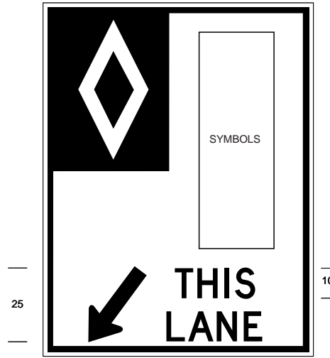
RESERVED LANE Sign (Multiple Vehicle Classes, Ground-mounted, No Days and Times)
