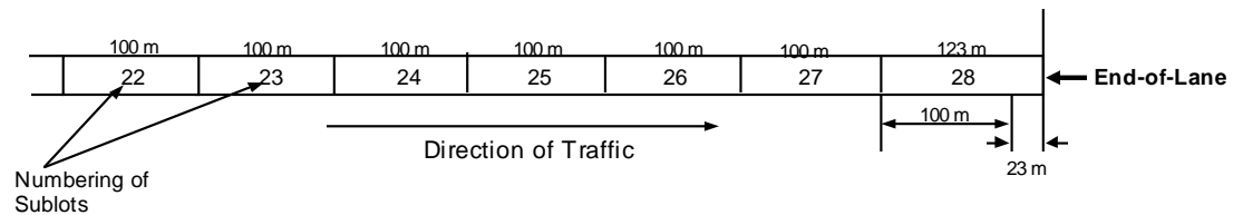
Figure 6-3: End-of-Lane Sublots
