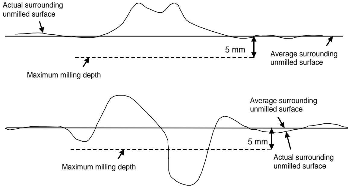
Figure 6-1: Diamond Grinding or Micromilling Limits
