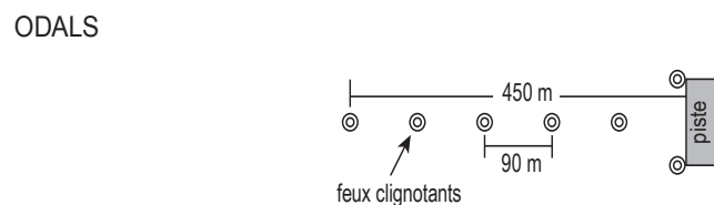
Figure 7.2 – ODALS
