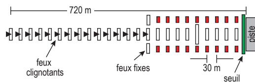
Figure 7.5 – ALSF-2
