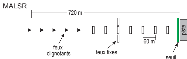
Figure 7.4 – MALSr
