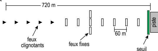
Figure 7.4 – MALSRL
