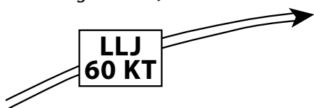
Figure 4.5h) – LLJ
