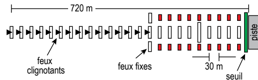
Figure 7.5 – ALSF-2
