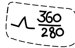
Figure 12.2e) – Turbulences
