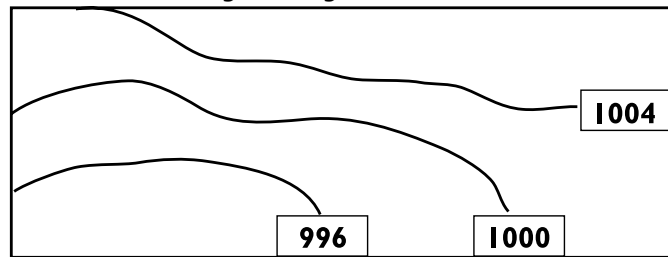
Figure 4.4g) – Isobares
