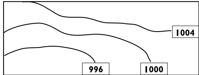
Figure 4.4g) – Isobares
