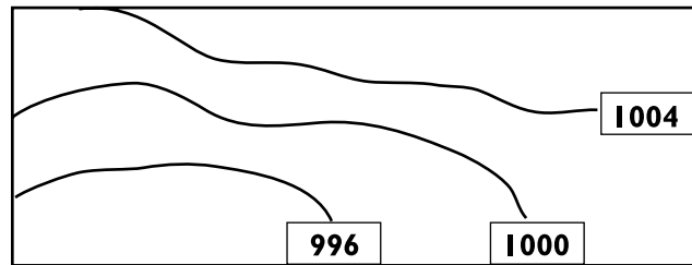
Figure 4.4g) – Isobares
