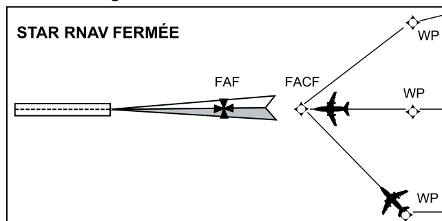
Figure 9.2 - STAR RNAV fermée
