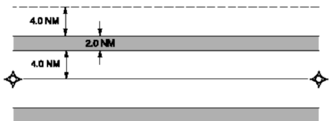
Figure 2.7a) – Route RNAV fixe
