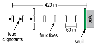
Figure 7.3 – MALSF
