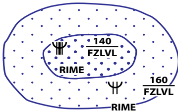
Figure 4.5c) – Givrage fort
