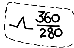
Figure 12.2e) – Turbulences
