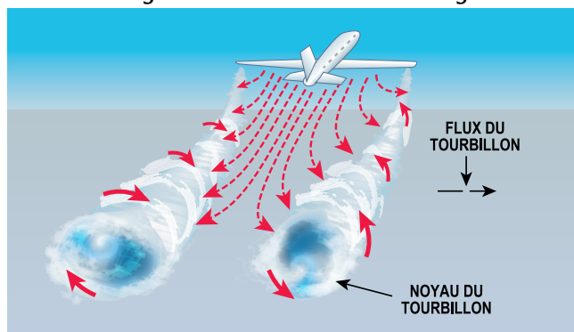
Figure 2.7 - Turbulence de sillage
