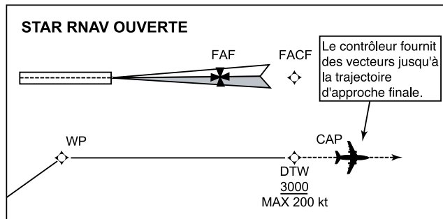
Figure 9.1 - STAR RNAV ouverte
