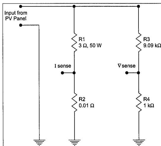
Figure 8. Half bridge network.
