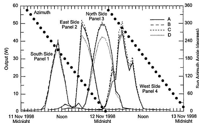
Figure 11. PV panel performance on the high-visibility day (11 to 12 January 1998) over 24 hours.
