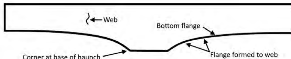
Figure 120. Illustration. Haunched girder.
