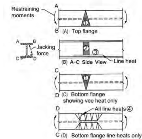
Figure 36. Illustration. Heating pattern and sequence for weak axis bending and local flange bulge.
