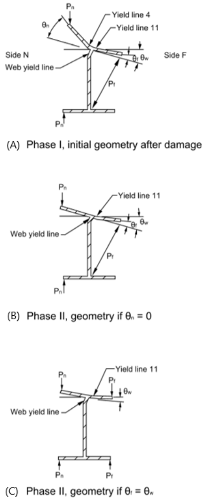
Figure 111. Illustration. Jacking sequence if damage is reversed from that shown in figure 109.
