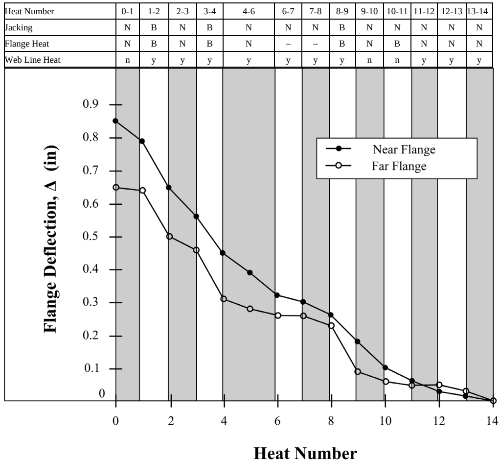
Figure 107. Graph. Flange movements for various heating patterns, beam no. 4 with category L/U damage (N and B refer to near and both sides of the flange, respectively; y and n refer to yes and no, respectively).
