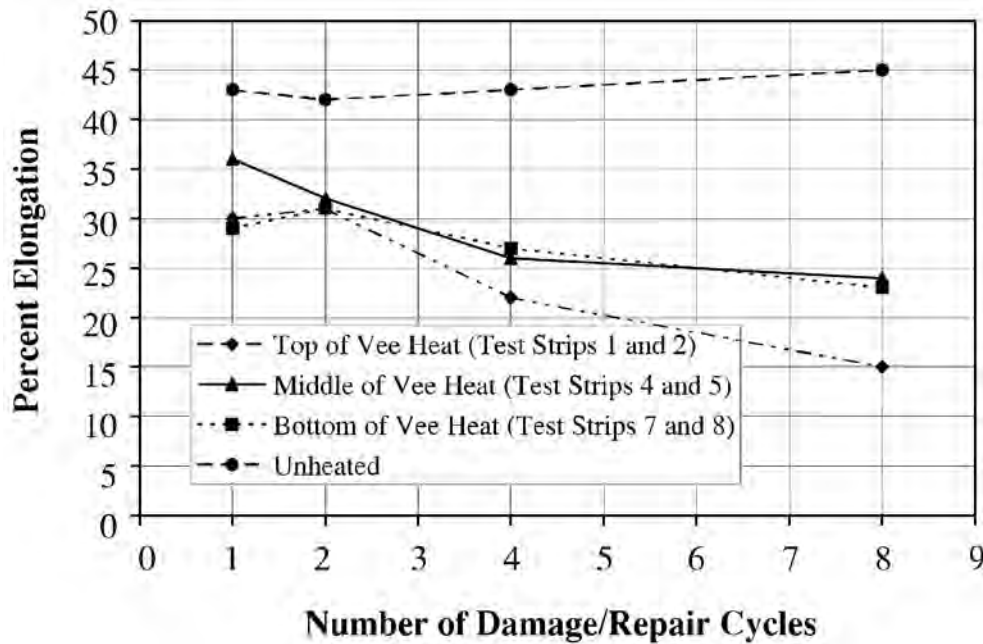
Figure 16. Graph. Percent elongation versus number of damage/repair cycles.
