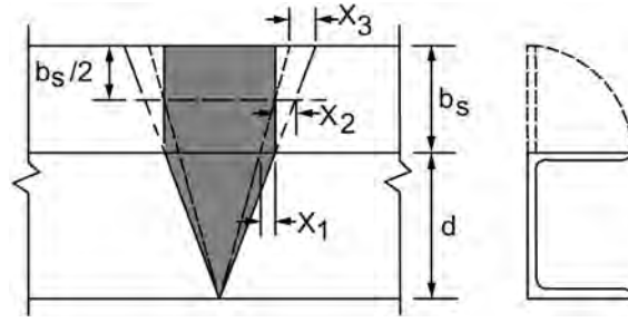
Figure 73. Illustration. Unfolded flange for a channel with category S damage.
