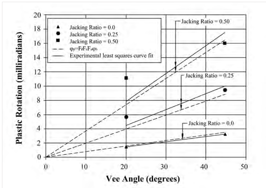
Figure 85. Graph. Influence of vee angle and jacking ratio on plastic rotation for L4×4×1/4 angles using the heating pattern shown in figure 84-A.
