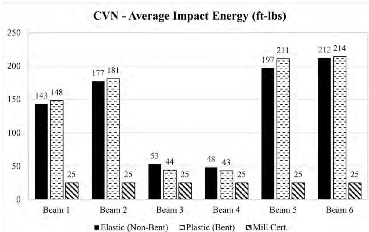
Figure 136. Graph. CVN values for cold bent beams.
