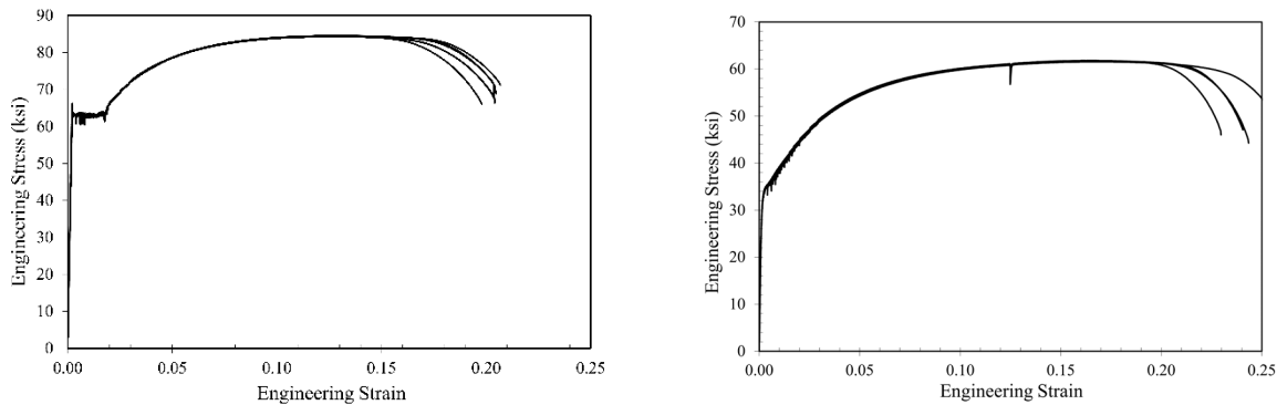
A. Stress-strain curve (with yield plateau)
