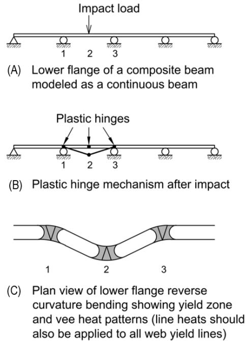
Figure 92. Illustration. Lower flange of composite girder modeled as a continuous beam.
