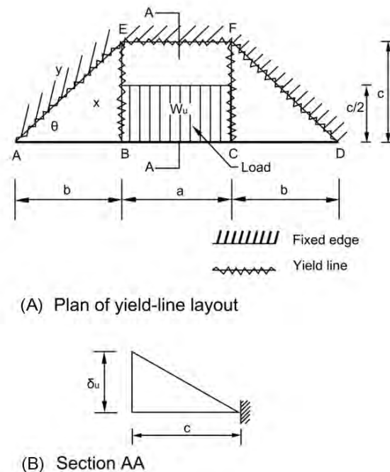
Figure 112. Illustration. Yield-line analysis for idealized flange bulge geometry.
