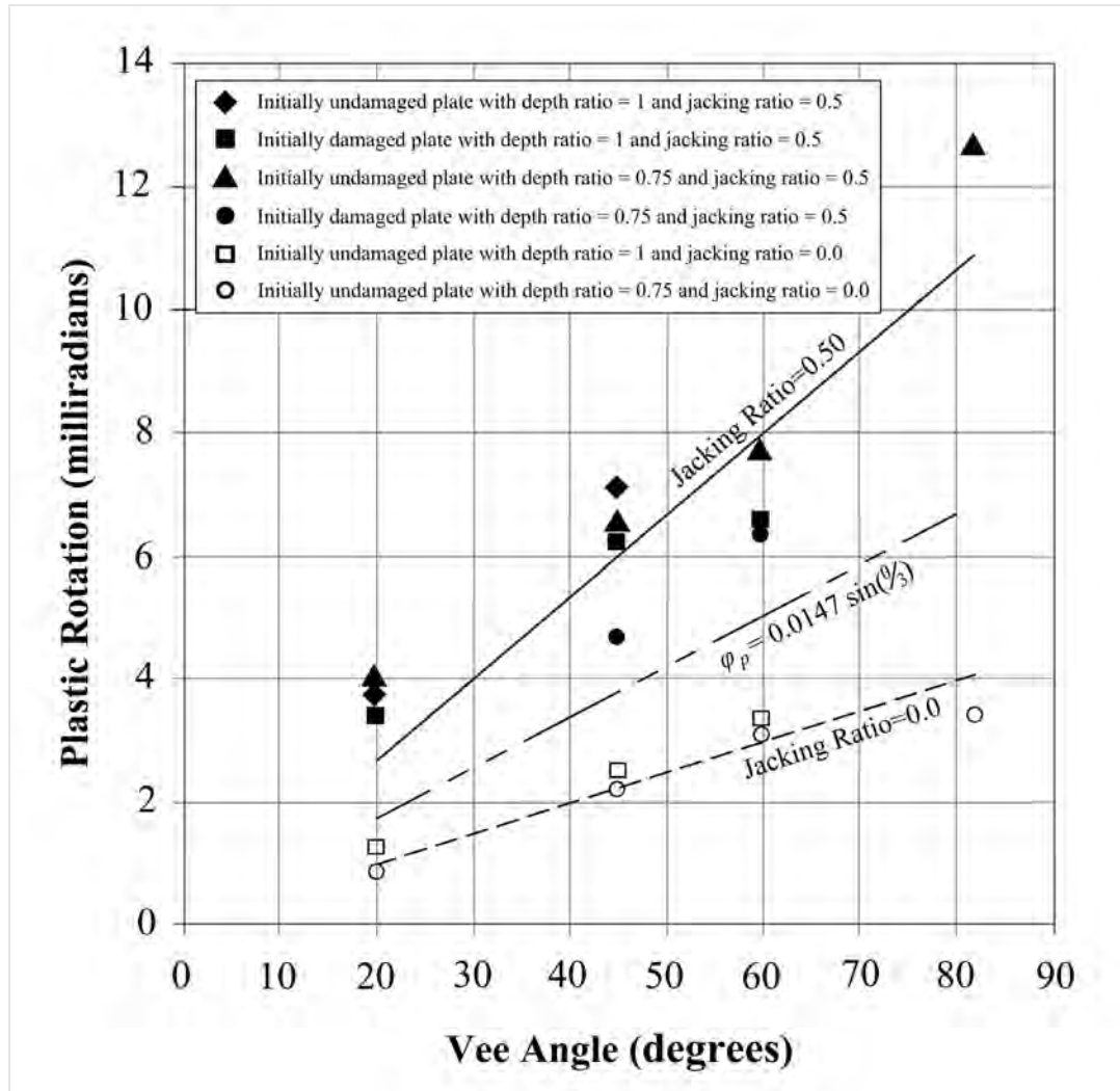
Figure 67. Graph. Plastic rotation versus vee angle for vee-heated plates having a heating temperature of 1,200°F.
