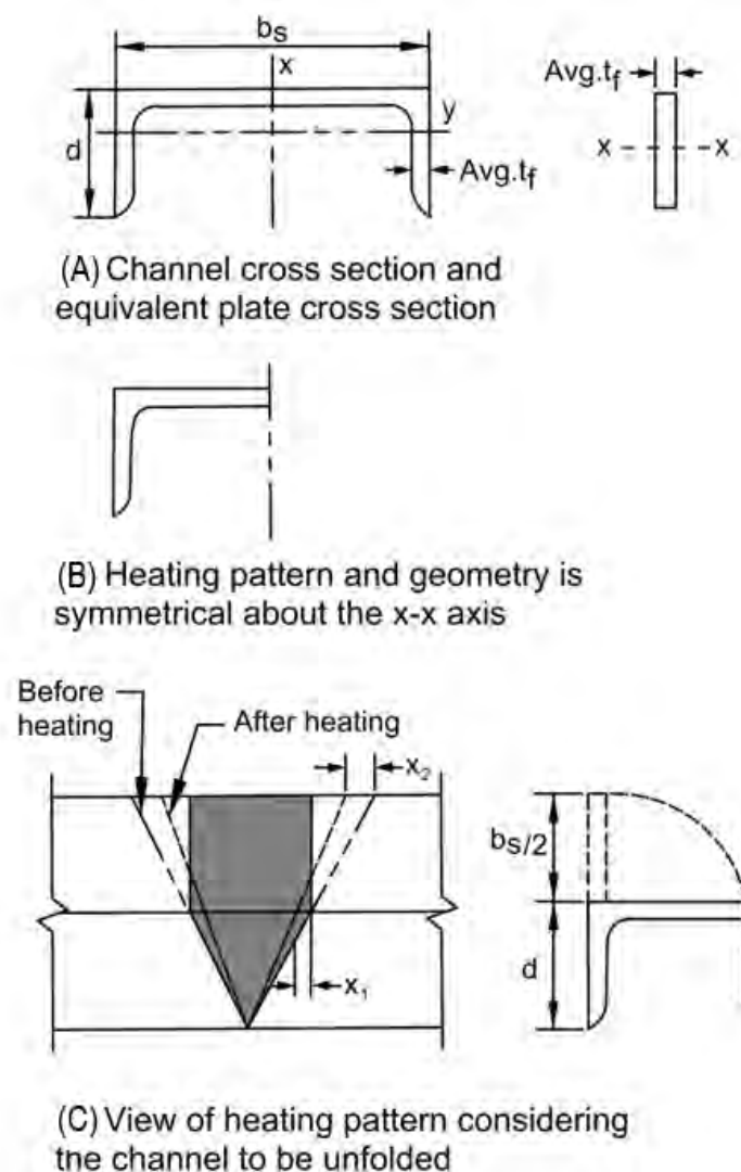
Figure 76. Illustration. Geometric effects on heat straightening a channel with negative curvature damage (as shown in figure 74-A).
