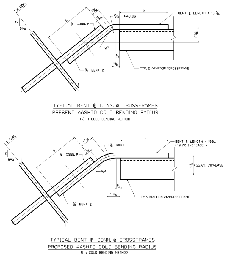
Figure 138. Illustration. Minimum radius effect on work points.
