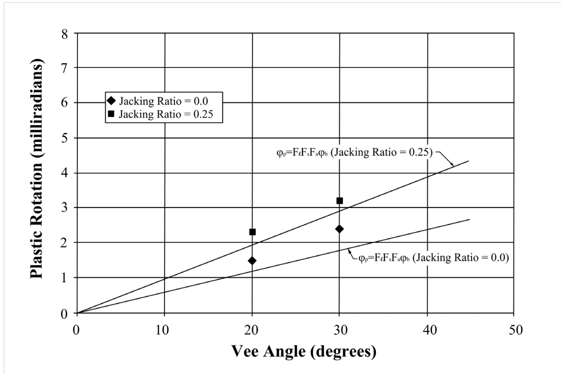
Figure 82. Graph. Influence of vee angle and jacking ratio on plastic rotation for W12×14 beam with category S damage.
