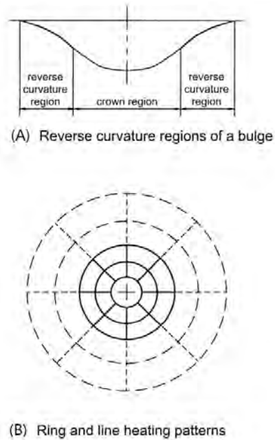
Figure 117. Illustration. Curvature and line heating patterns for category L/S damage.
