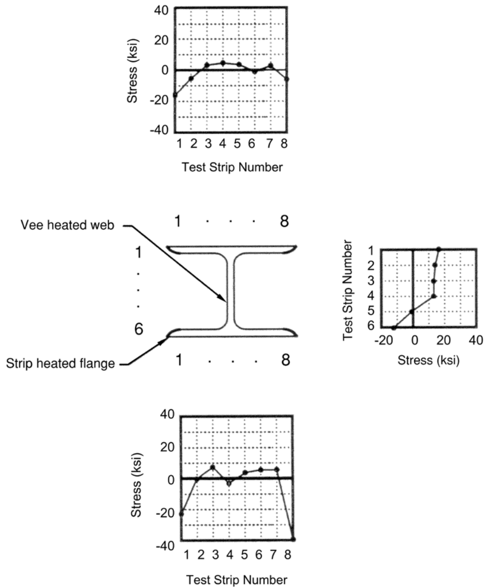
Figure 9. Illustration. Typical residual stress distribution for a Category S heat-straightened wide flange beam.
