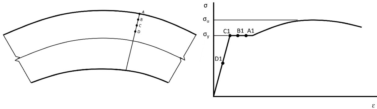
A. Bent plate B. Stress-strain curve
