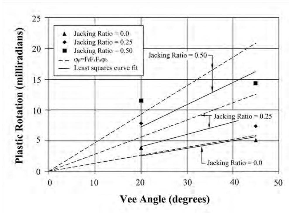
Figure 75. Graph. Experimental and theoretical plastic rotations for a C6×8.2 channel with category W damage (with the open end of vees at flange-web-juncture).
