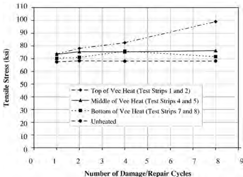
Figure 15. Graph. Tensile stress versus number of damage/repair cycles.
