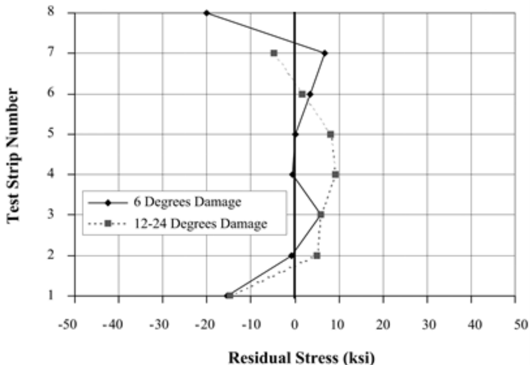
Figure 5. Graph. Residual stress distribution for plates damaged and then vee-heated.
