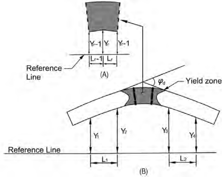
Figure 40. Illustration. Offset measurements to calculate angle of damage and radius of curvature.
