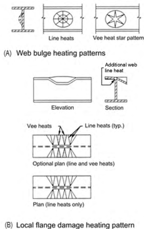
Figure 33. Illustration. Typical heating patterns for local damage.
