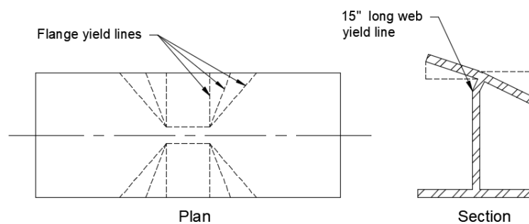
(B) Yield zones for typical flange bulge
