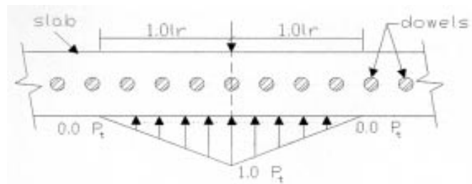
Figure 3.67 : Distribution de la charge [Davis, 1998]
