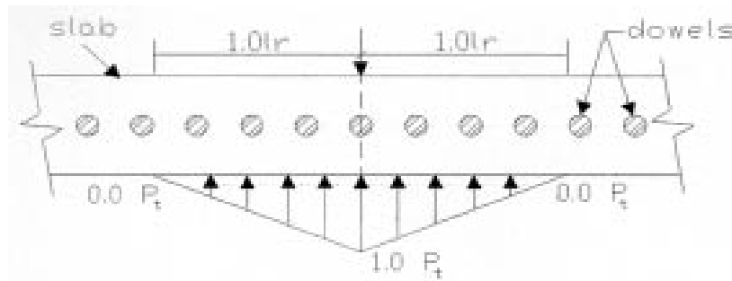
Figure 2.11 : Distribution de la charge [Davis, 1998]
