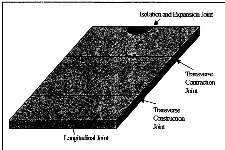
Figure 2.4 : Types et disposition des joints [Eddie, 1999]
