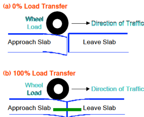
Figure 2.8 : Illustration du transfert de charge [Smith, 2001]
