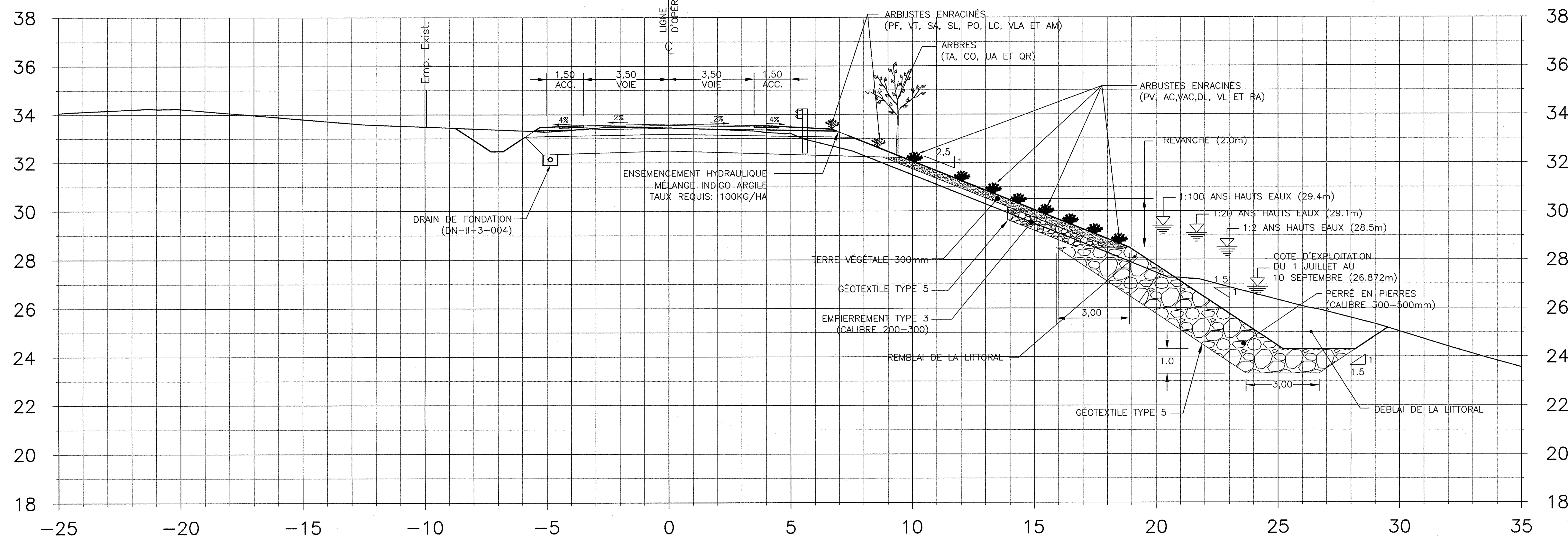
ROUTE 231 COUPE TRANSVERSALE CH. 2+200
