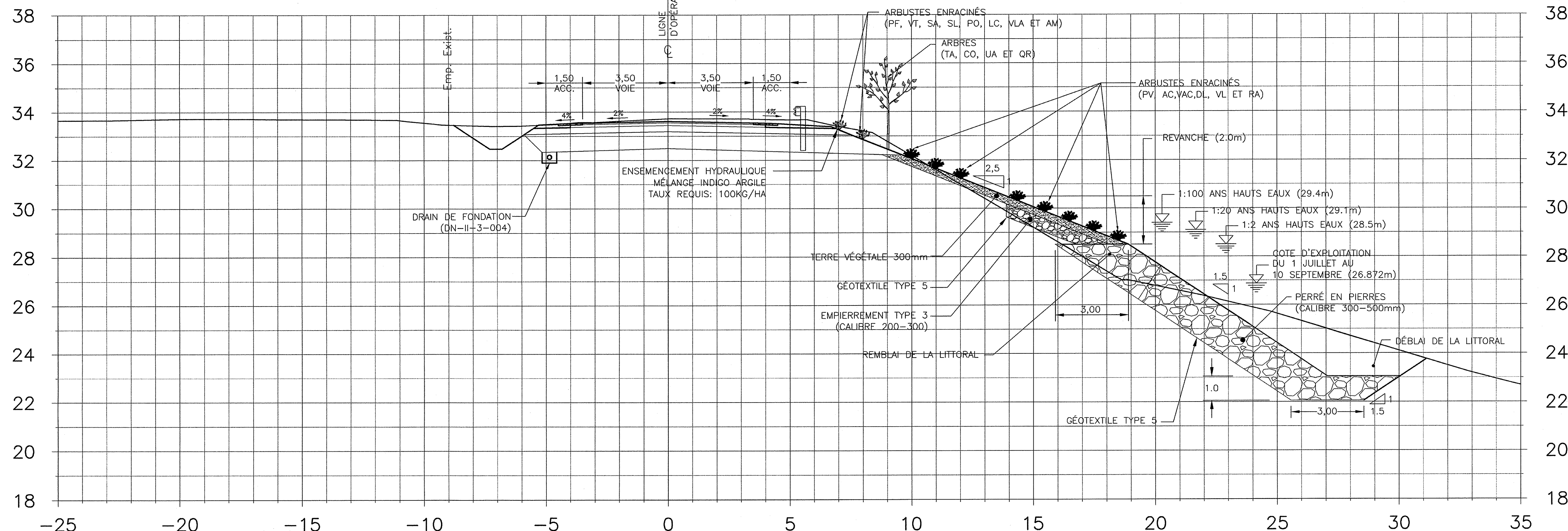
ROUTE 231 COUPE TRANSVERSALE CH. 1+780
