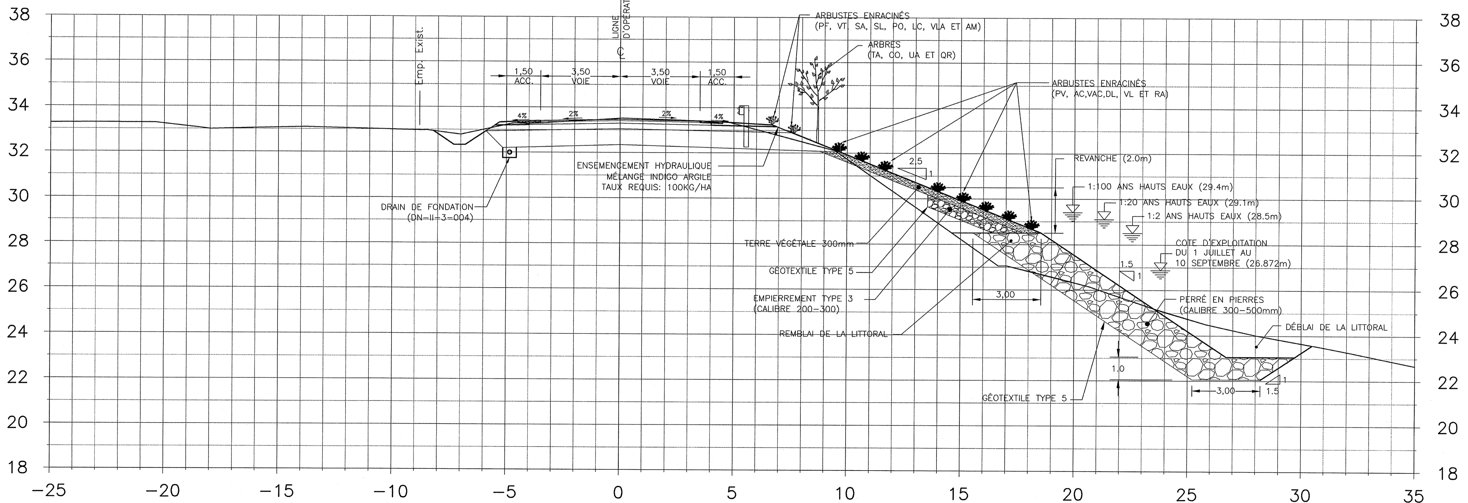
ROUTE 231 COUPE TRANSVERSALE CH. 1+740
