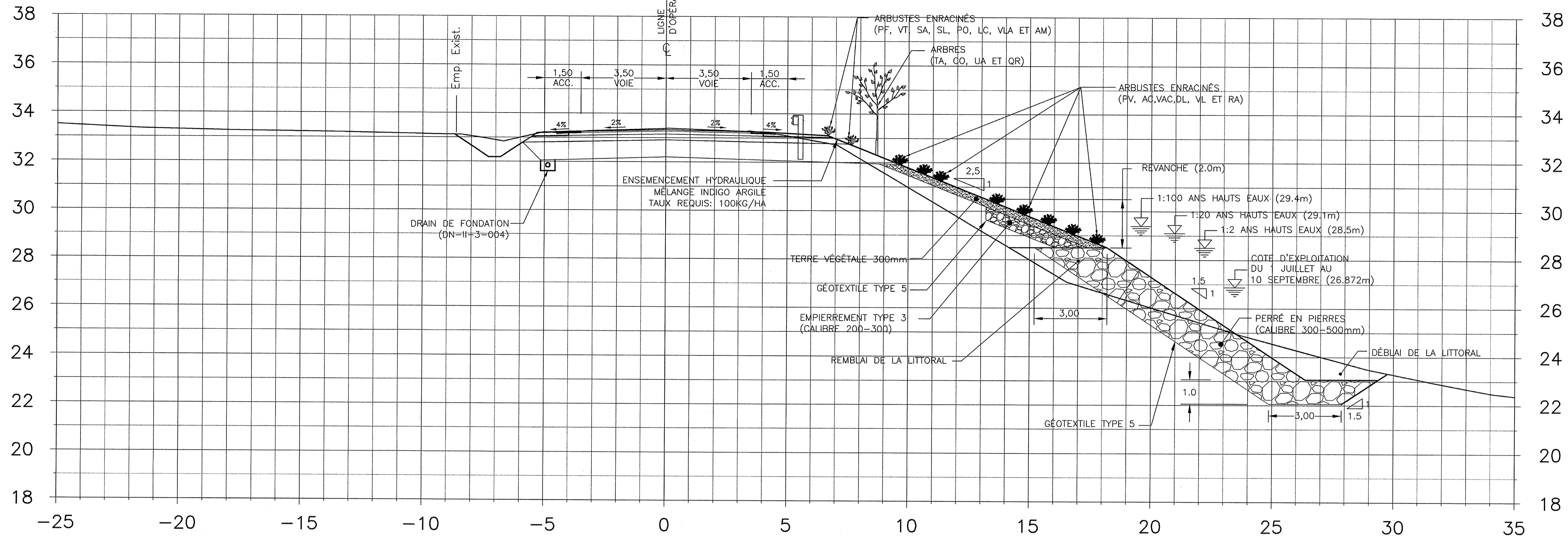
ROUTE 231 COUPE TRANSVERSALE CH. 1+700
