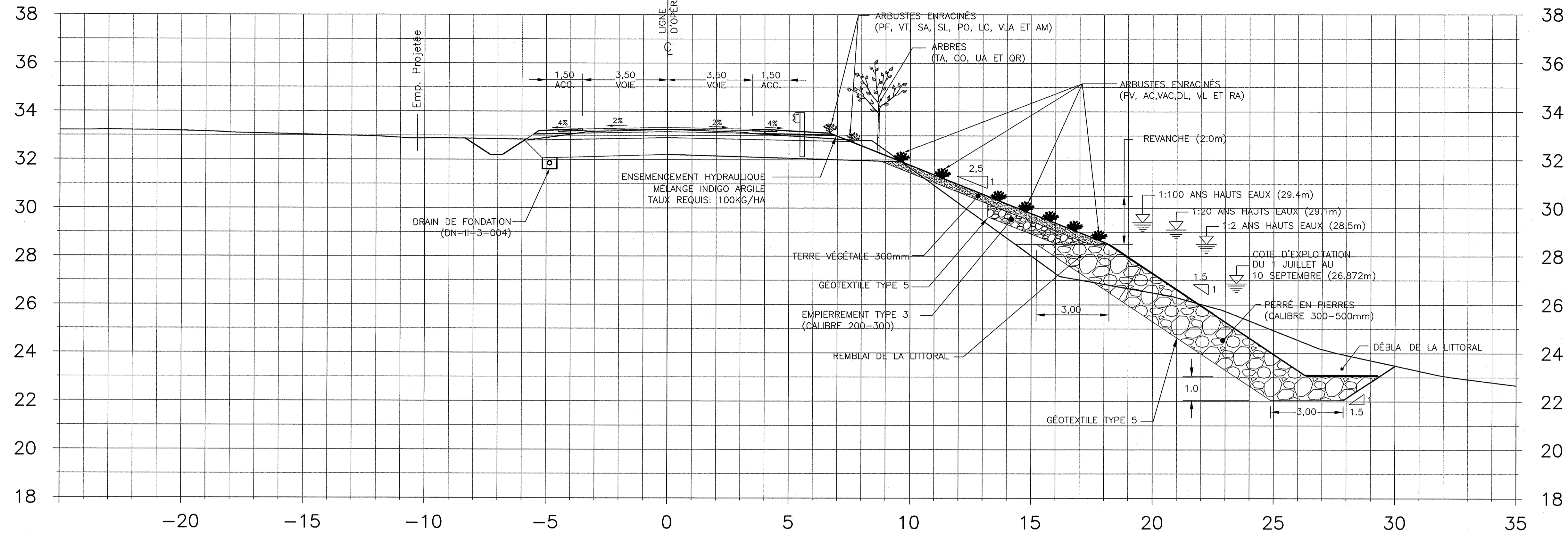
ROUTE 231 COUPE TRANSVERSALE CH. 1+380
