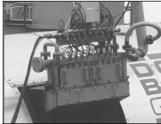
Figure 3b: Foam Injection System
