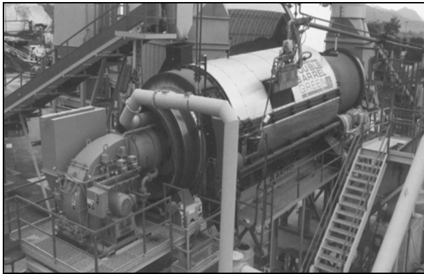
Figure 3a: Double Barrel Green Plant
