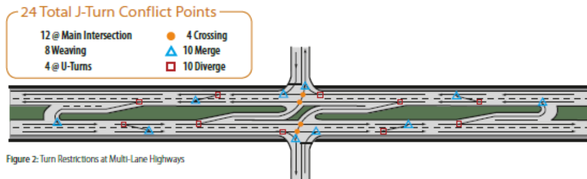
Figure 4: Turn Restrictions at Multi-Lane Highways
