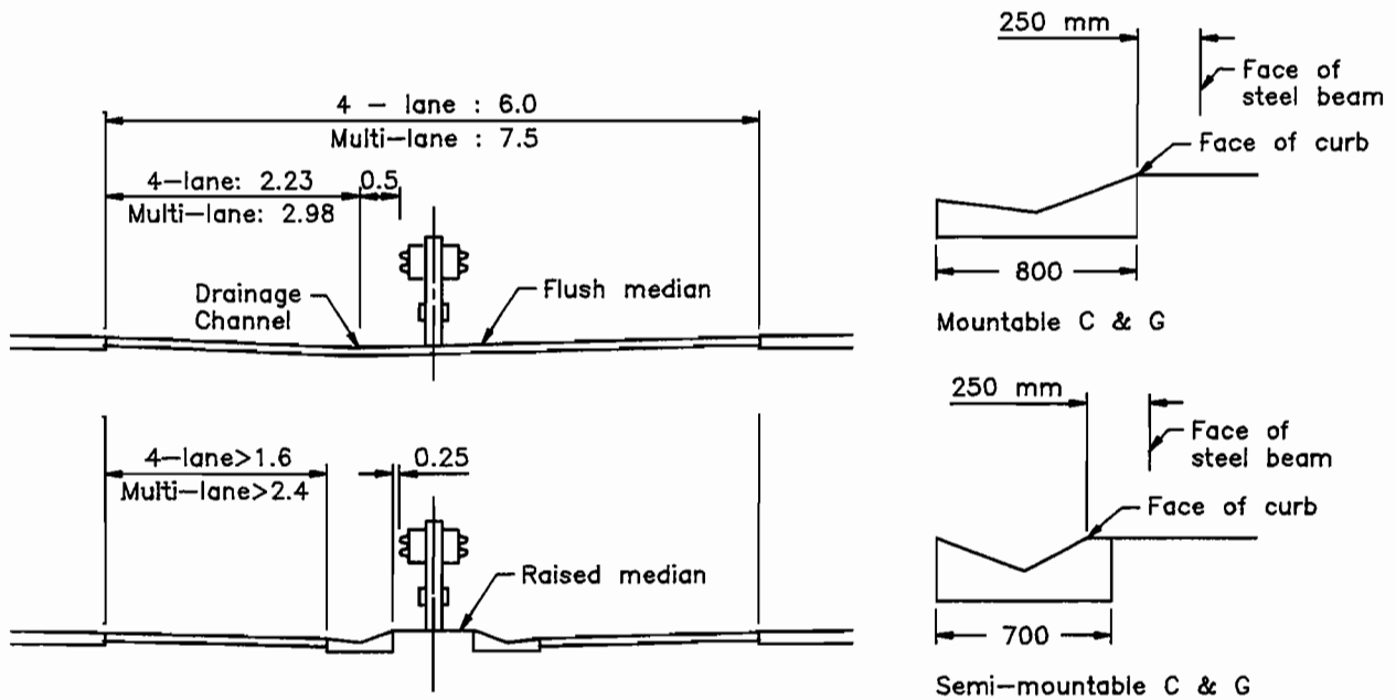
Double Steel Beam Barrier (a) Without Bridge Pier
