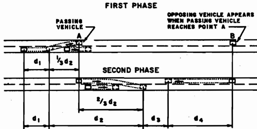
Figure C2-1 PASSING MANOEUVRE
