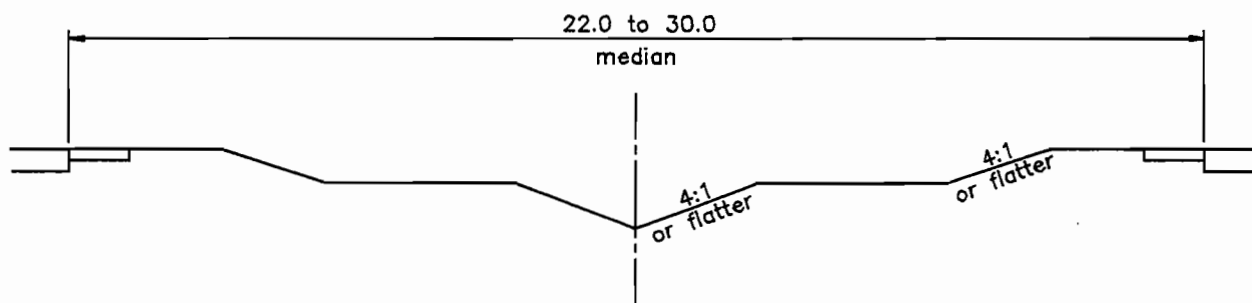
Figure D6-1 Median Width for Rural Freeways
