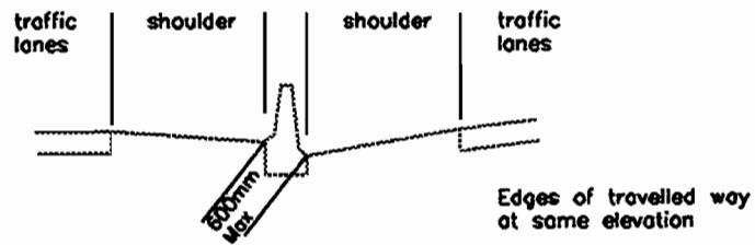
NARROW MEDIAN
