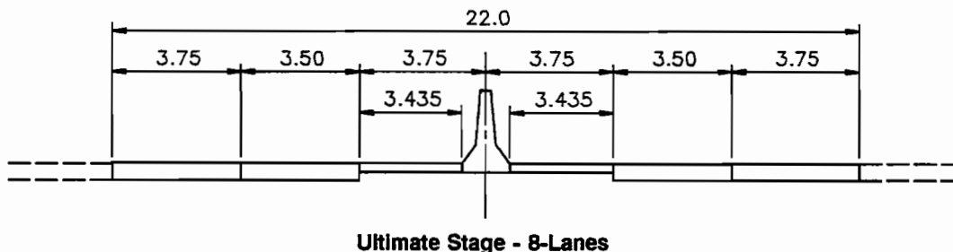
Ultimate Stage - 8-Lanes
