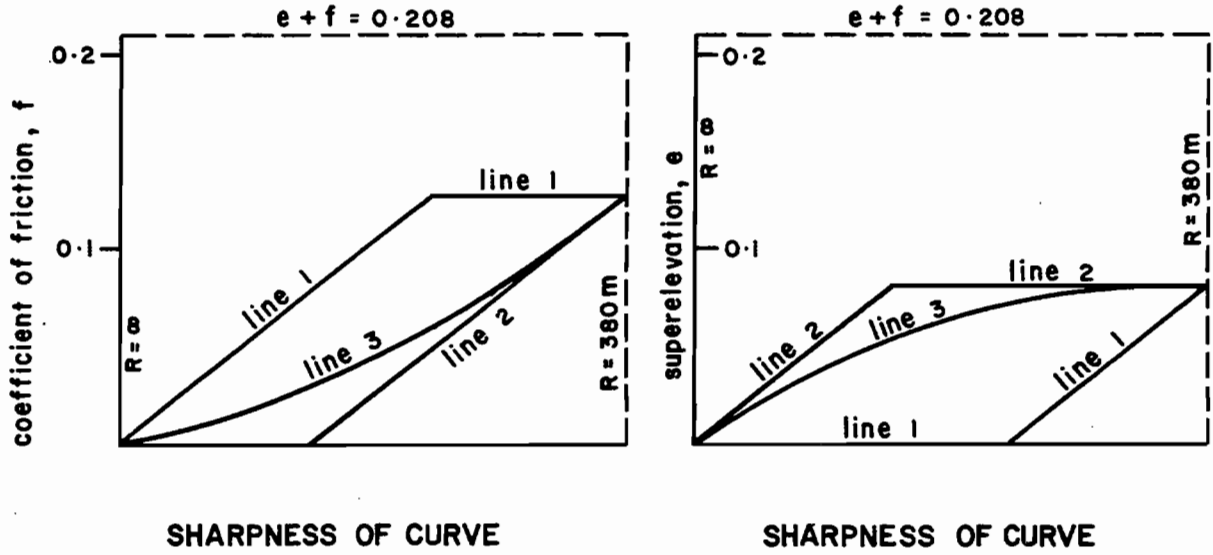
Figure C3-1 Distribution of Superelevation
