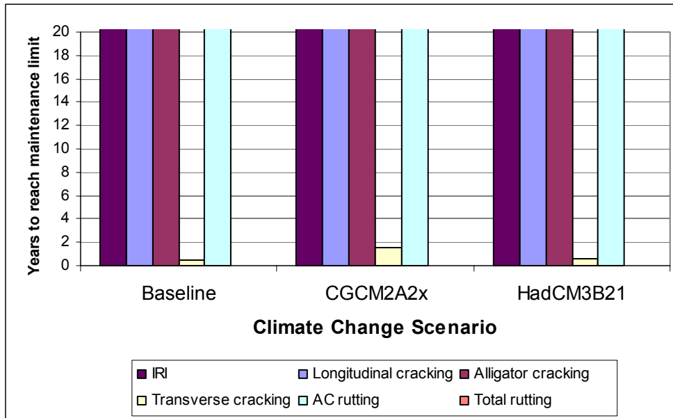
Figure 33a. Years to reach performance parameter limits (50% reliability maintenance thresholds) under no traffic growth scenario at the Newfoundland site (St. John's)
