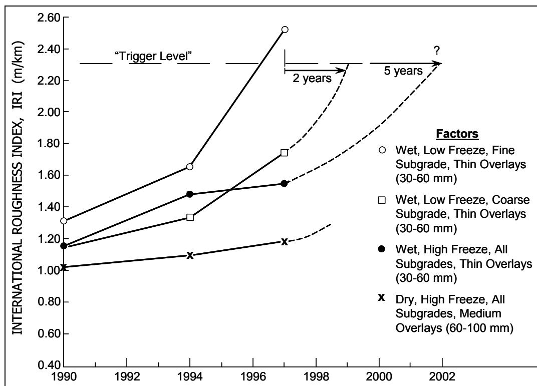
Figure 6. Roughness progression comparisons from Canadian strategic highway research program, Long Term Pavement Performance (C-LTPP) experiment (Tighe et al., 2001)
