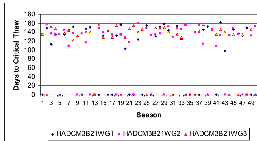
Figure B-26. Kelowna estimated days to critical TI (HadCM3B21 scenario series)
