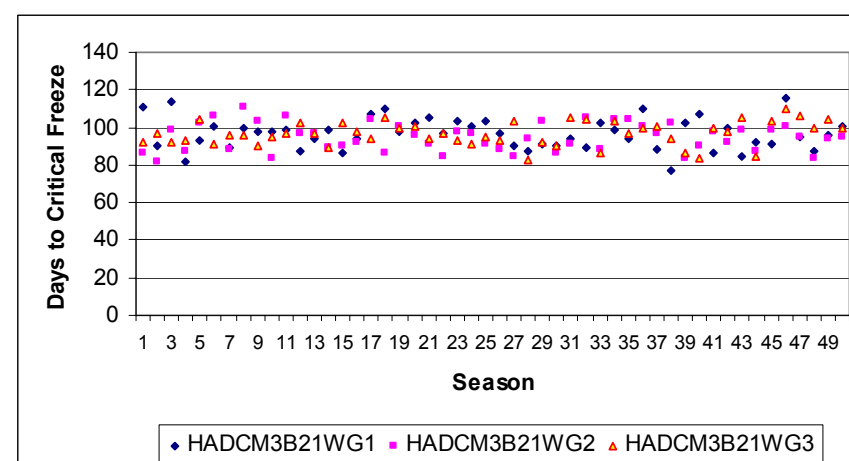
Figure B-233. Montreal estimated days to critical FI (HadCM3B21 scenario series)
