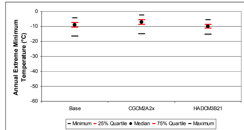
Figure B-7. Vancouver annual extreme minimum temperature distribution: quartile statistics (n=150)
