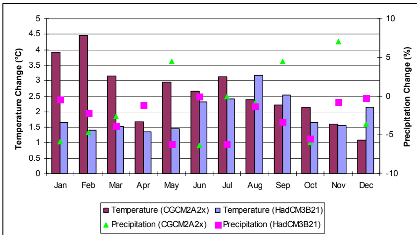
Figure 32. CGCM2A2x and HadCM3B21 temperature and precipitation change scenarios (2050s) for the Newfoundland site (St. John's)
