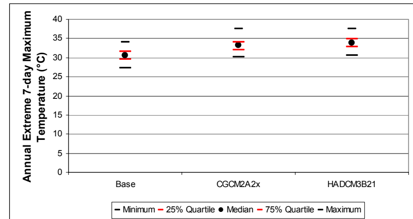
Figure B-187. Toronto annual extreme 7-day mean maximum daily temperature distribution: quartile statistics (n=150)
