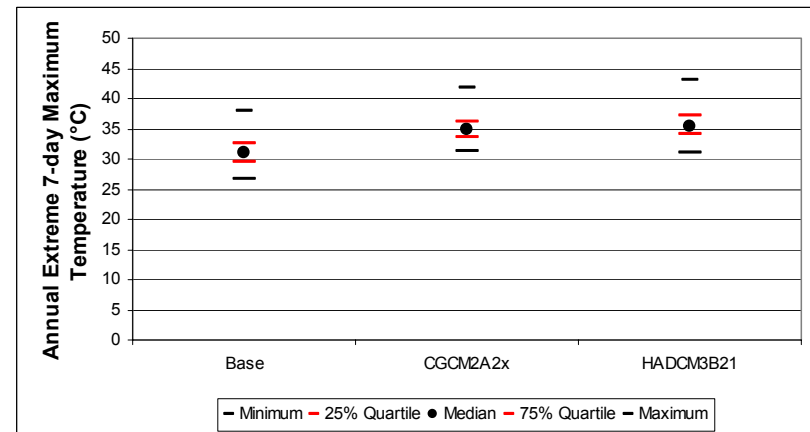
Figure B-77. Regina annual extreme 7-day mean maximum daily temperature distribution: quartile statistics (n=150)
