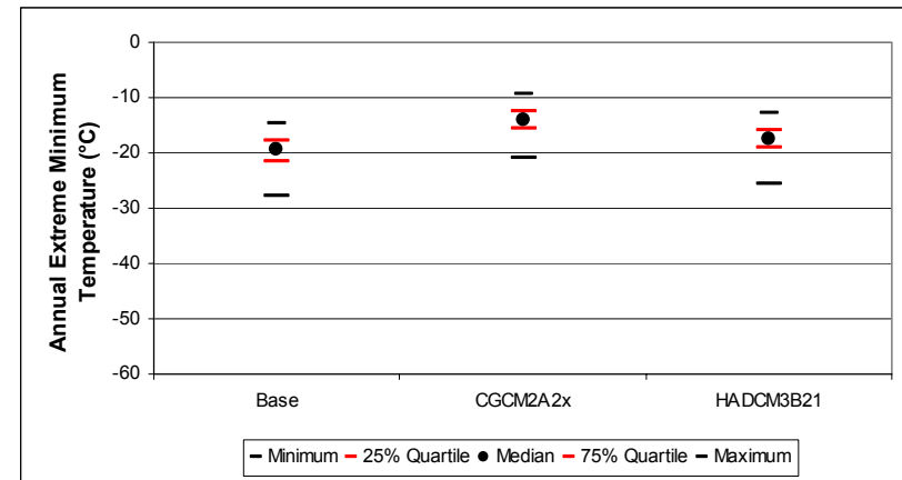
Figure B-306. St. John's annual extreme minimum temperature distribution: quartile statistics (n=150)
