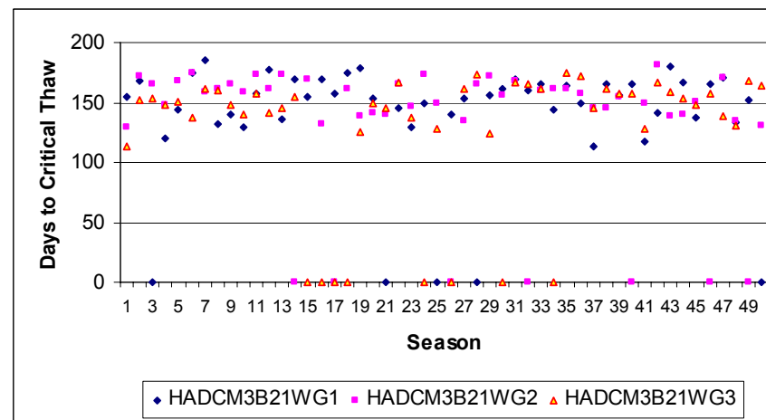
Figure B-296. Halifax estimated days to critical TI (HadCM3B21 scenario series)
