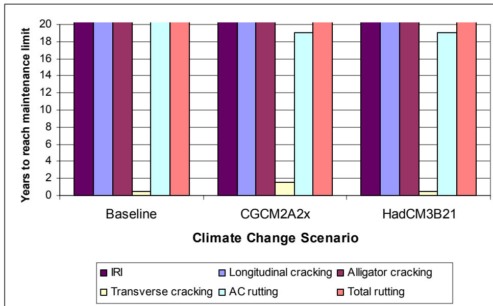
Figure D-43. Years to reach performance parameter limits (50% reliability maintenance thresholds) under 4 percent annual traffic growth scenario at the Ontario site (Toronto)
