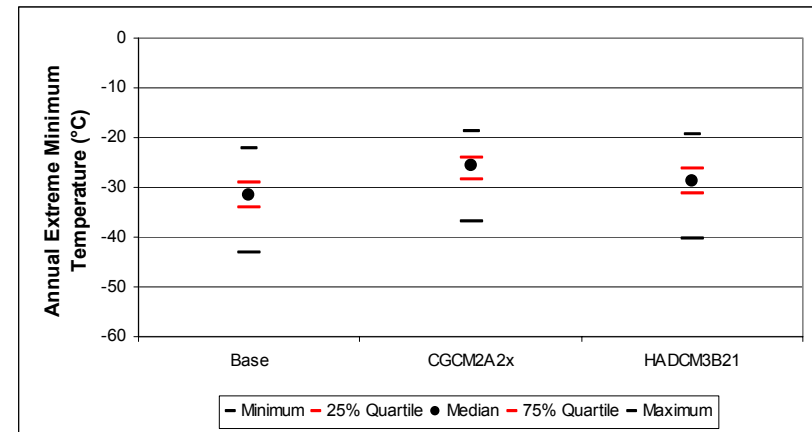
Figure B-266. Fredericton annual extreme minimum temperature distribution: quartile statistics (n=150)
