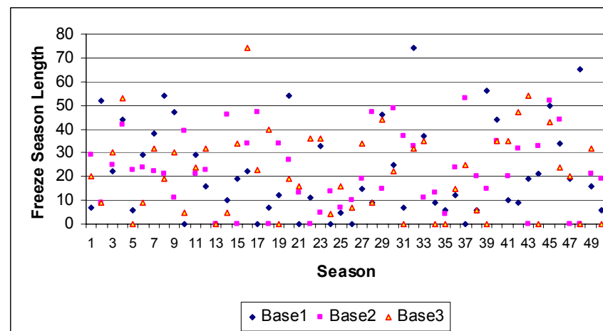
Figure B-27. Kelowna estimated freeze season length (baseline series)
