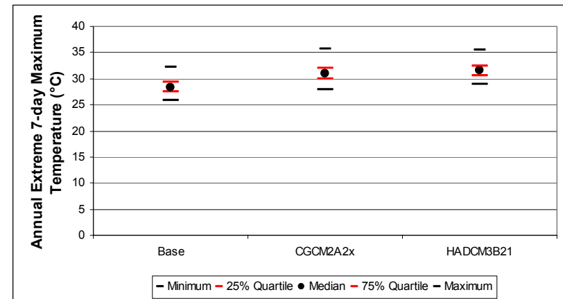
Figure B-147. Muskoka annual extreme 7-day mean maximum daily temperature distribution: quartile statistics (n=150)
