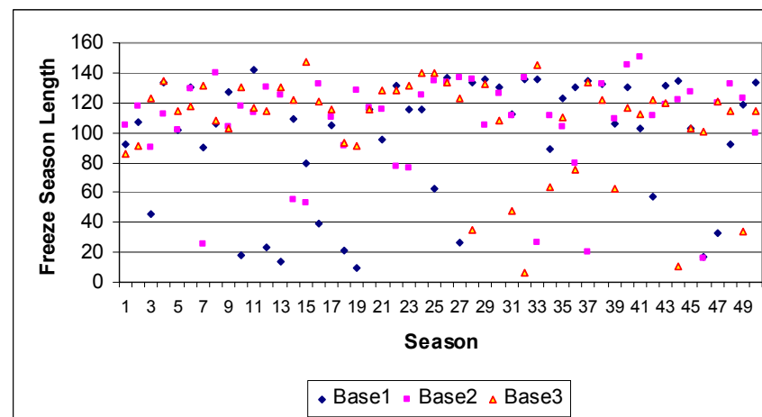
Figure B-67. Edmonton estimated freeze season length (baseline series)
