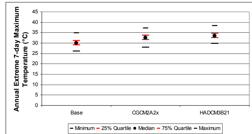
Figure B-207. Ottawa annual extreme 7-day mean maximum daily temperature distribution: quartile statistics (n=150)
