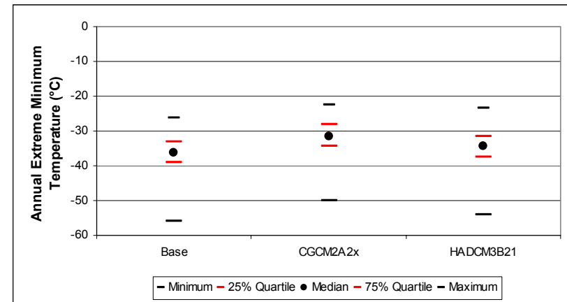
Figure B-36. Calgary annual extreme minimum temperature distribution: quartile statistics (n=150)
