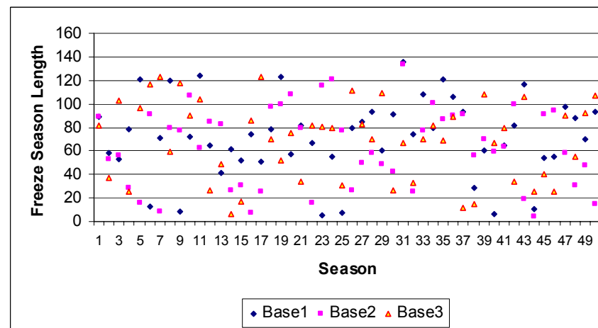
Figure B-47. Calgary estimated freeze season length (baseline series)
