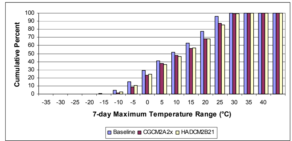
Figure B-124. North Bay 7-day means maximum daily temperature cumulative percent distribution (n=54750)
