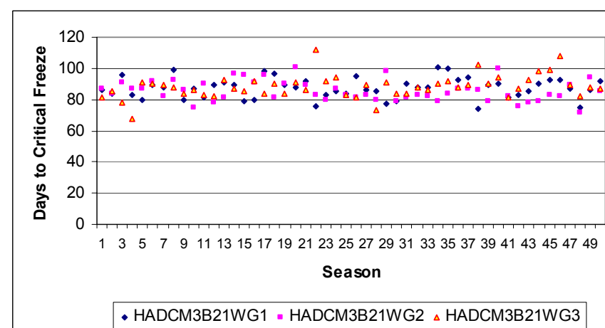
Figure B-253. Quebec estimated days to critical FI (HadCM3B21 scenario series)
