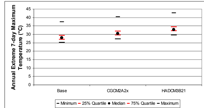
Figure B-37. Calgary annual extreme 7-day mean maximum daily temperature distribution: quartile statistics (n=150)
