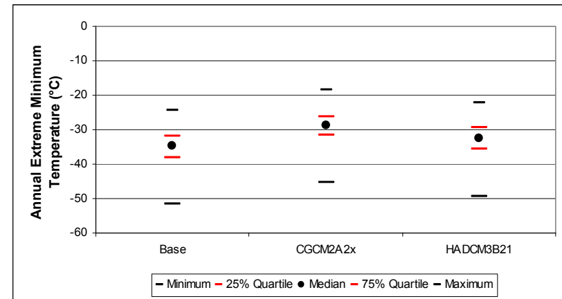
Figure B-146. Muskoka annual extreme minimum temperature distribution: quartile statistics (n=150)
