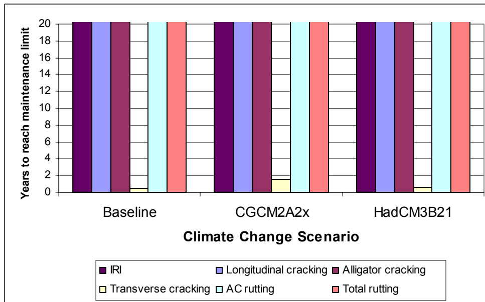
Figure D-47. Years to reach performance parameter limits (50% reliability maintenance thresholds) under 4 percent annual traffic growth scenario at the Newfoundland site (St. John's)
