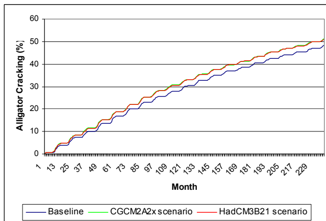
Figure D-15. Alligator cracking performance at the Manitoba site (Winnipeg) under baseline and future climate scenarios assuming 0(left) and 4(right) percent annual increase in traffic
