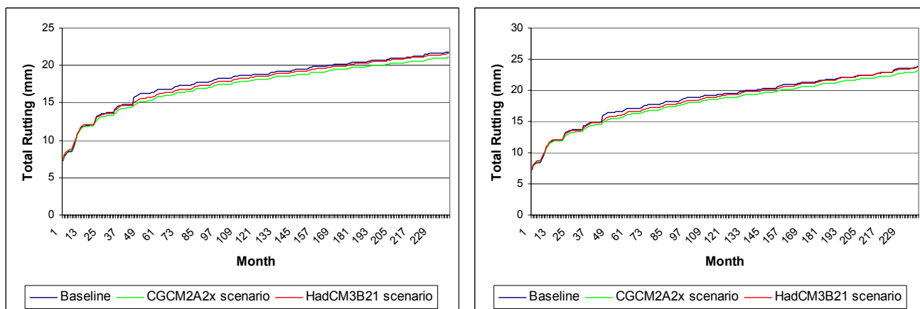
Figure D-30. Total rutting performance at the Quebec site (Montreal) under baseline and future climate scenarios assuming 0(left) and 4(right) percent annual increase in traffic
