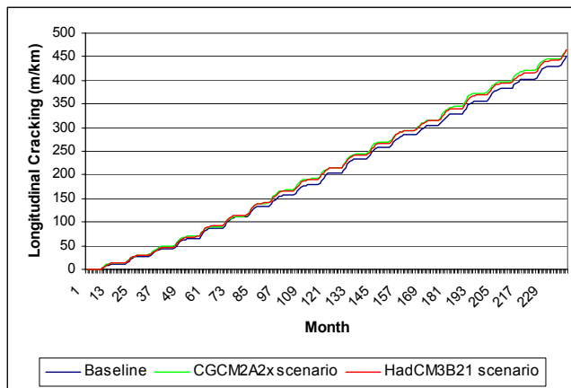
Figure D-14. Longitudinal cracking performance at the Manitoba site (Winnipeg) under baseline and future climate scenarios assuming 0(left) and 4(right) percent annual increase in traffic
