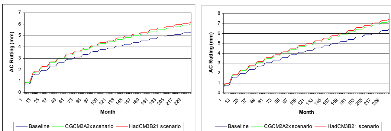
Figure D-29. AC rutting performance at the Quebec site (Montreal) under baseline and future climate scenarios assuming 0(left) and 4(right) percent annual increase in traffic
