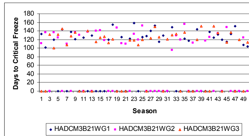
Figure B-173. Windsor estimated days to critical FI (HadCM3B21 scenario series)
