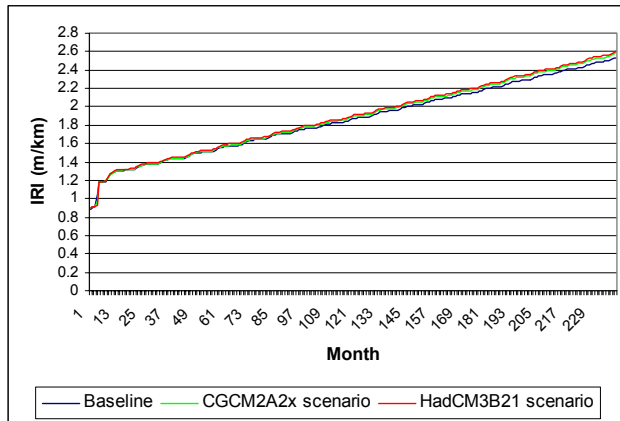
Figure D-13. IRI performance at the Manitoba site (Winnipeg) under baseline and future climate scenarios assuming 0(left) and 4(right) percent annual increase in traffic
