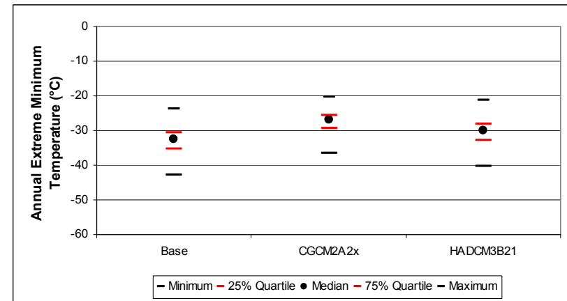
Figure B-246. Quebec annual extreme minimum temperature distribution: quartile statistics (n=150)
