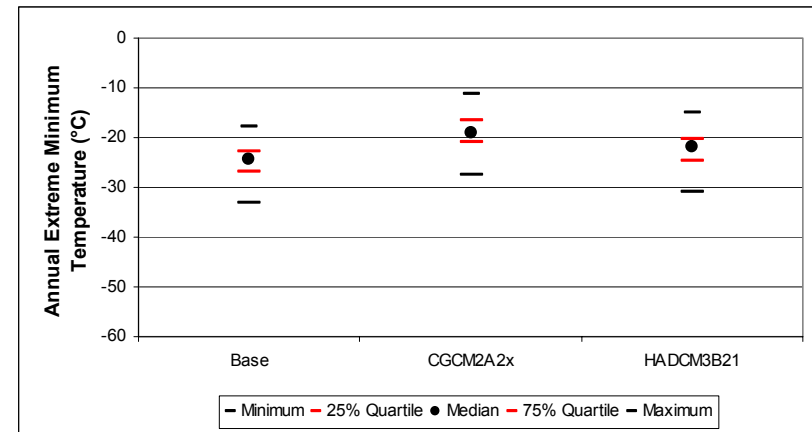
Figure B-186. Toronto annual extreme minimum temperature distribution: quartile statistics (n=150)
