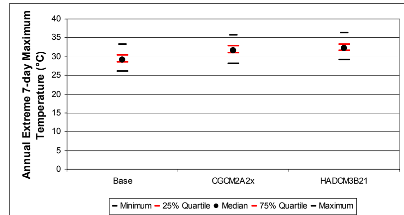
Figure B-267. Fredericton annual extreme 7-day mean maximum daily temperature distribution: quartile statistics (n=150)
