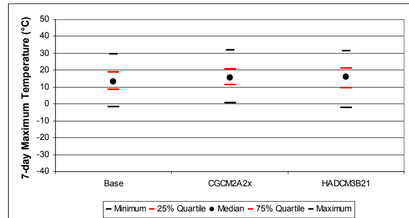
Figure B-6. Vancouver 7-day mean maximum daily temperature distribution: quartile statistics (n=54750)
