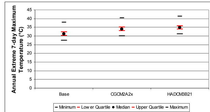
Figure B-167. Windsor annual extreme 7-day mean maximum daily temperature distribution: quartile statistics (n=150)
