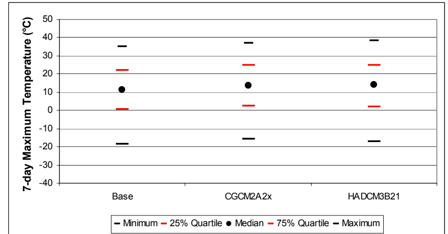
Figure B-205. Ottawa 7-day mean maximum daily temperature distribution: quartile statistics (n=54750)
