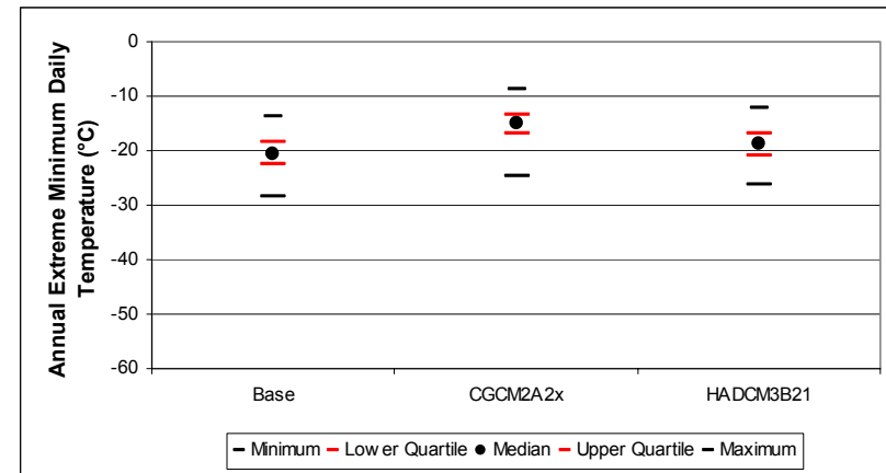
Figure B-166. Windsor annual extreme minimum temperature distribution: quartile statistics (n=150)
