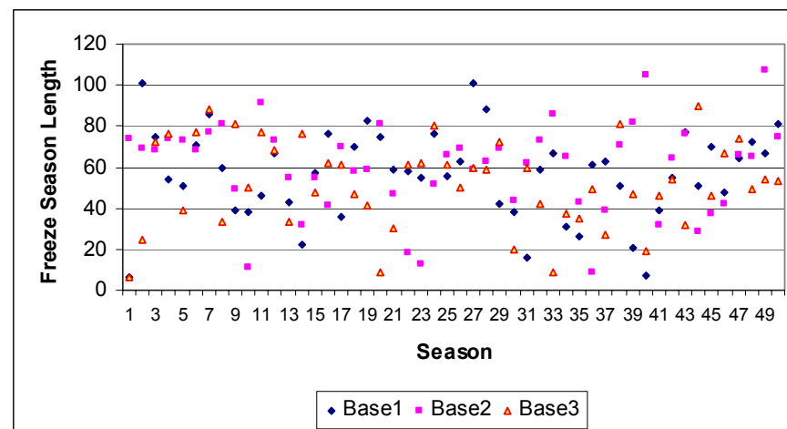
Figure B-317. St. John's estimated freeze season length (baseline series)
