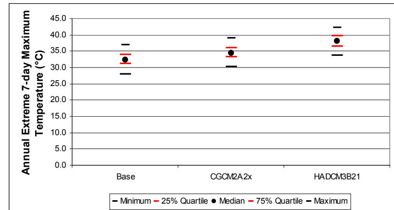
Figure B-17. Kelowna annual extreme 7-day mean maximum daily temperature distribution: quartile statistics (n=150)
