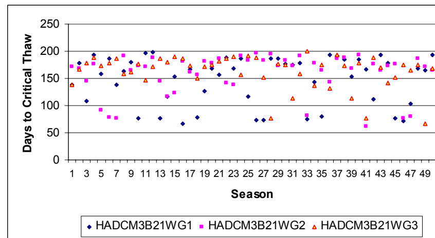
Figure B-66. Edmonton estimated days to critical TI (HadCM3B21 scenario series)
