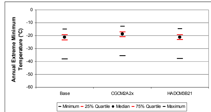
Figure B-16. Kelowna annual extreme minimum temperature distribution: quartile statistics (n=150)
