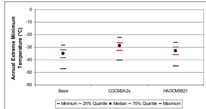
Figure B-126. North Bay annual extreme minimum temperature distribution: quartile statistics (n=150)
