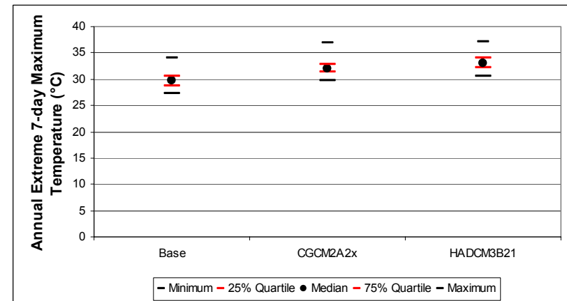
Figure B-227. Montreal annual extreme 7-day mean maximum daily temperature distribution: quartile statistics (n=150)
