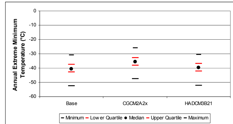
Figure B-86. Winnipeg annual extreme minimum temperature distribution: quartile statistics (n=150)
