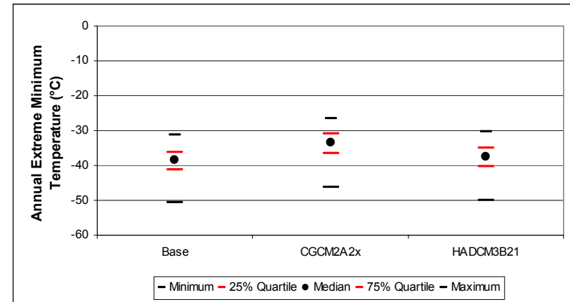
Figure B-106. Thunder Bay annual extreme minimum temperature distribution: quartile statistics (n=150)
