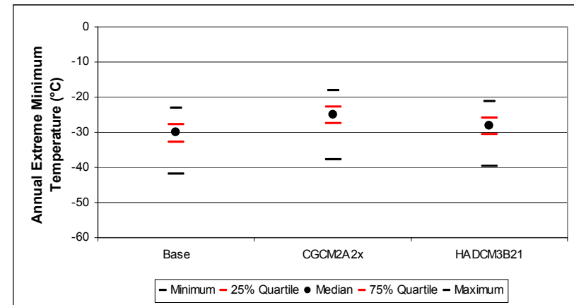
Figure B-206. Ottawa annual extreme minimum temperature distribution: quartile statistics (n=150)
