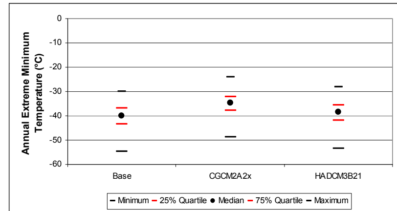
Figure B-56. Edmonton annual extreme minimum temperature distribution: quartile statistics (n=150)
