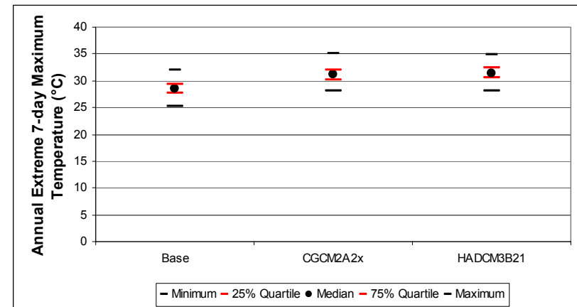
Figure B-247. Quebec annual extreme 7-day mean maximum daily temperature distribution: quartile statistics (n=150)
