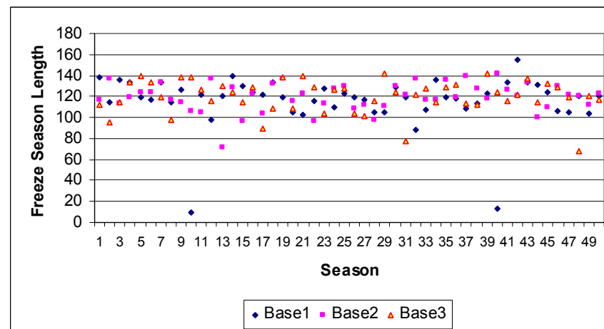
Figure B-87. Regina estimated freeze season length (baseline series)
