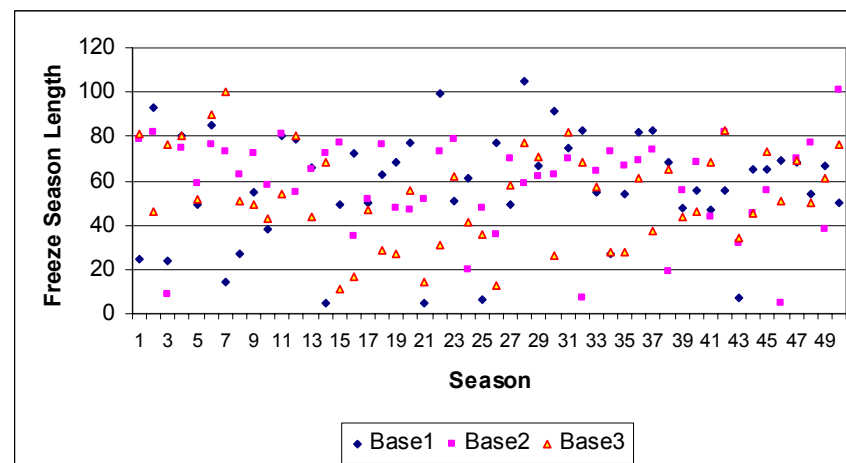
Figure B-297. Halifax estimated freeze season length (baseline series)
