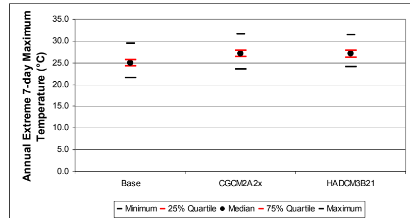
Figure B-8. Vancouver annual extreme 7-day mean maximum daily temperature distribution: quartile statistics (n=150)
