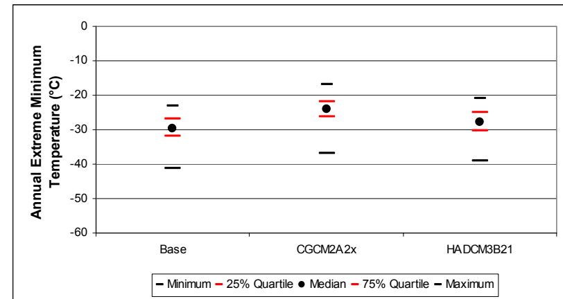
Figure B-226. Montreal annual extreme minimum temperature distribution: quartile statistics (n=150)
