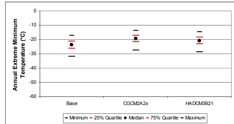
Figure B-286. Halifax annual extreme minimum temperature distribution: quartile statistics (n=150)
