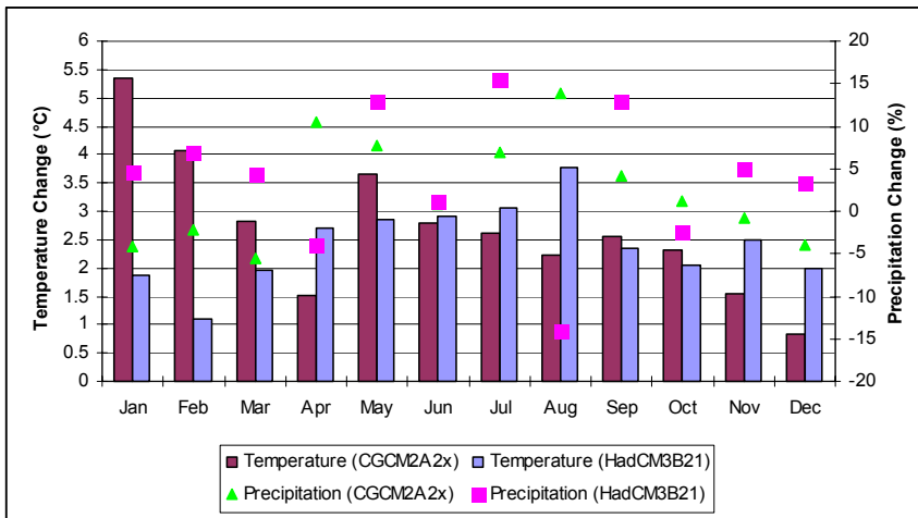
Figure 31. CGCM2A2x and HadCM3B21 temperature and precipitation change scenarios (2050s) for the Quebec site (Montreal)
