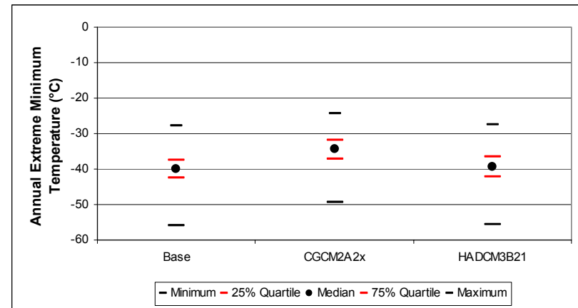
Figure B-76. Regina annual extreme minimum temperature distribution: quartile statistics (n=150)
