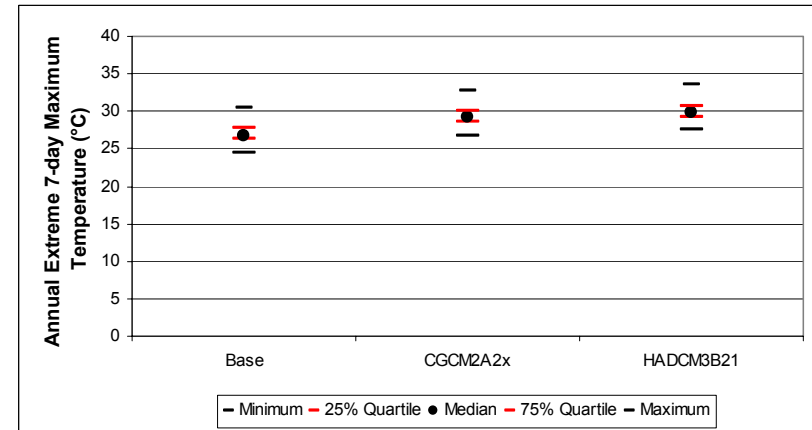
Figure B-287. Halifax annual extreme 7-day mean maximum daily temperature distribution: quartile statistics (n=150)
