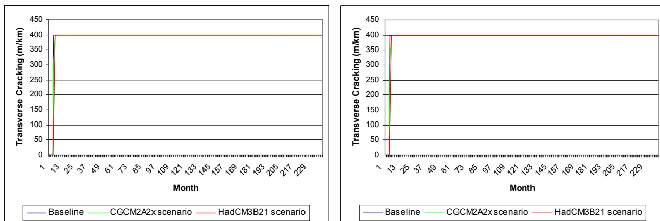
Figure D-28. Transverse cracking performance at the Quebec site (Montreal) under baseline and future climate scenarios assuming 0(left) and 4(right) percent annual increase in traffic
