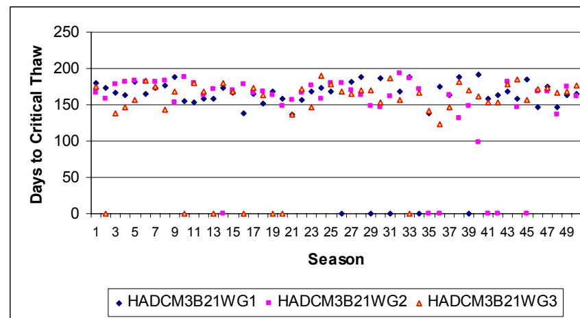
Figure B-316. St. John's estimated days to critical TI (HadCM3B21 scenario series)
