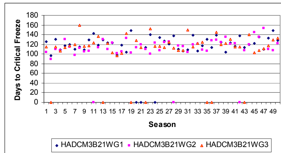
Figure B-193. Toronto estimated days to critical FI (HadCM3B21 scenario series)
