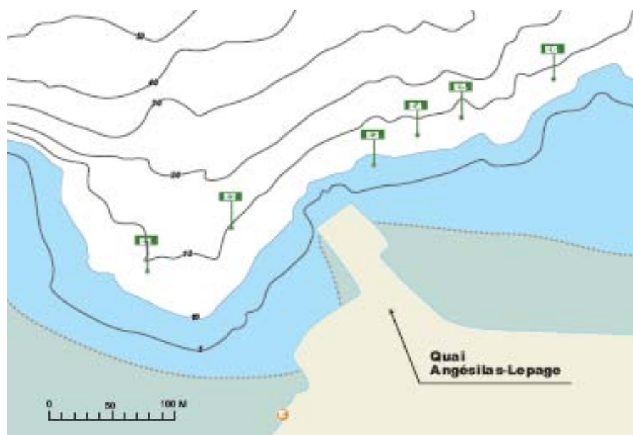
FIGURE 3 : BATHYMÉTRIE LOCALE
